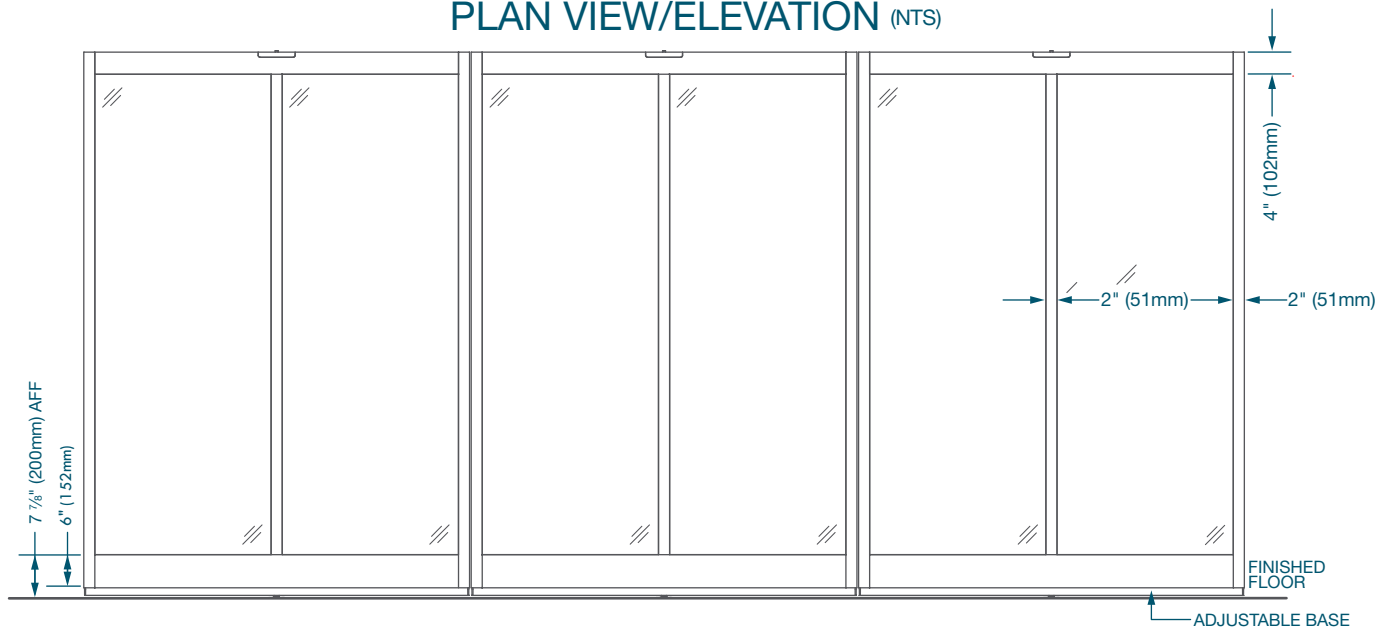
TRIPLE CENTER PIVOT DOOR FRAMED 2" STILE
