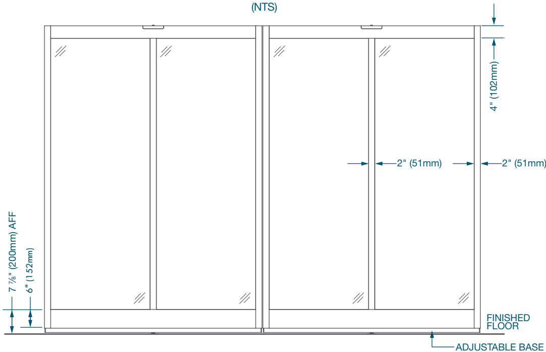
DOUBLE CENTER PIVOT DOOR FRAMED 2" STILE
