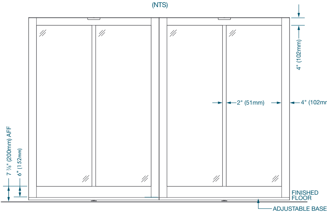
DOUBLE CENTER PIVOT DOOR FRAMED 4" STILE
