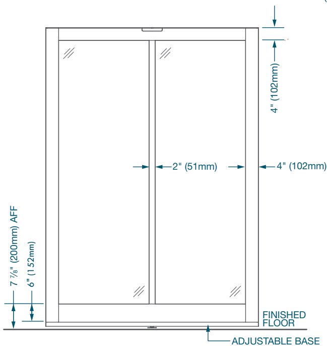
CENTER PIVOT DOOR FRAMED 4" STILE
