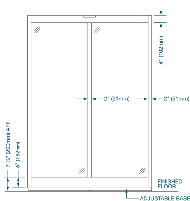
CENTER PIVOT DOOR FRAMED 2" STILE
