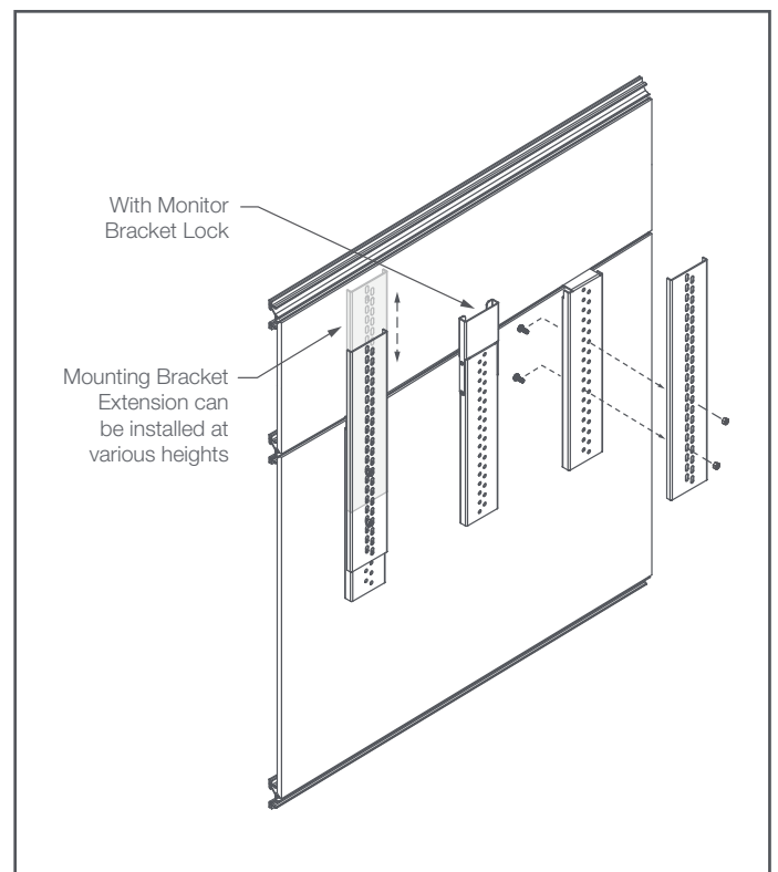
Figure 4. DIRT Mounting Bracket Extensions.
