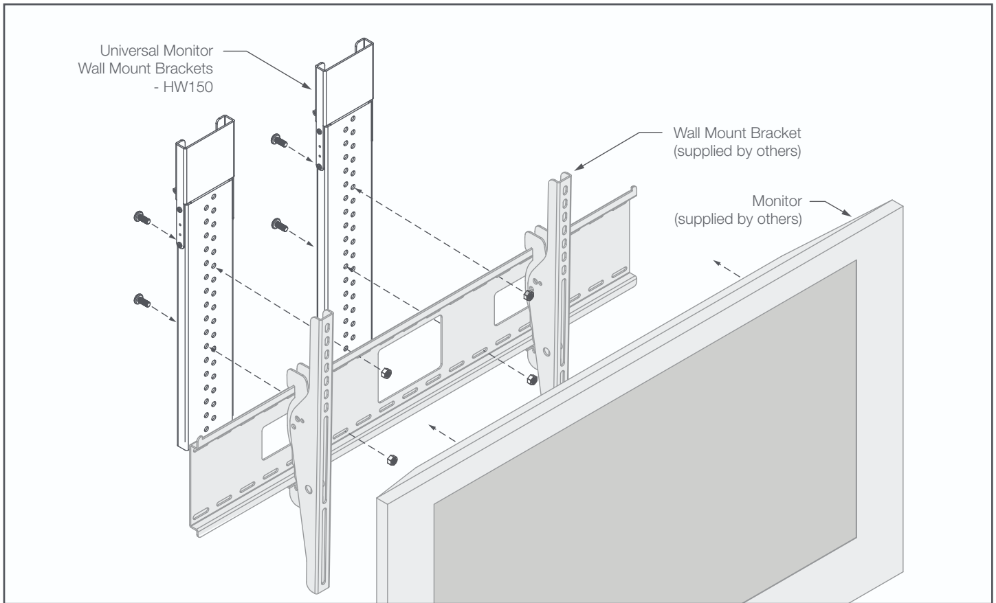
Figure 1. DIRT Universal TV Monitor Wall Mount Assembly.
