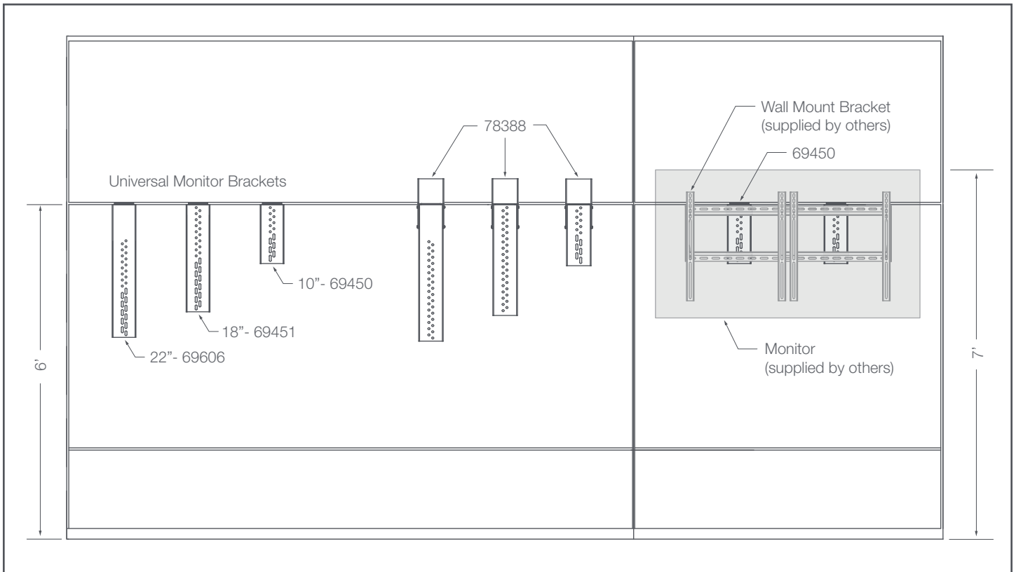
Figure 3. DIRT Universal TV Monitor Wall Mount Brackets.
