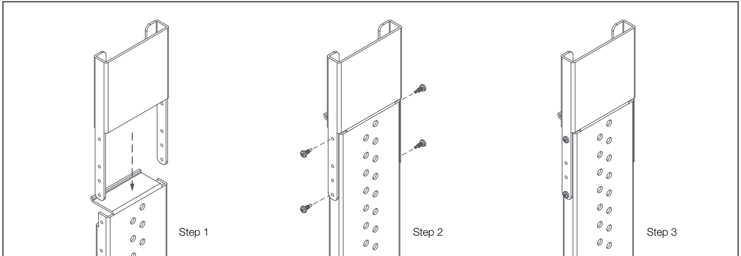
Figure 5. Assembling a TV Bracket Lock (HW274).
