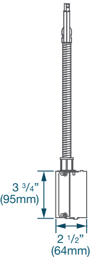
SIDE VIEW
