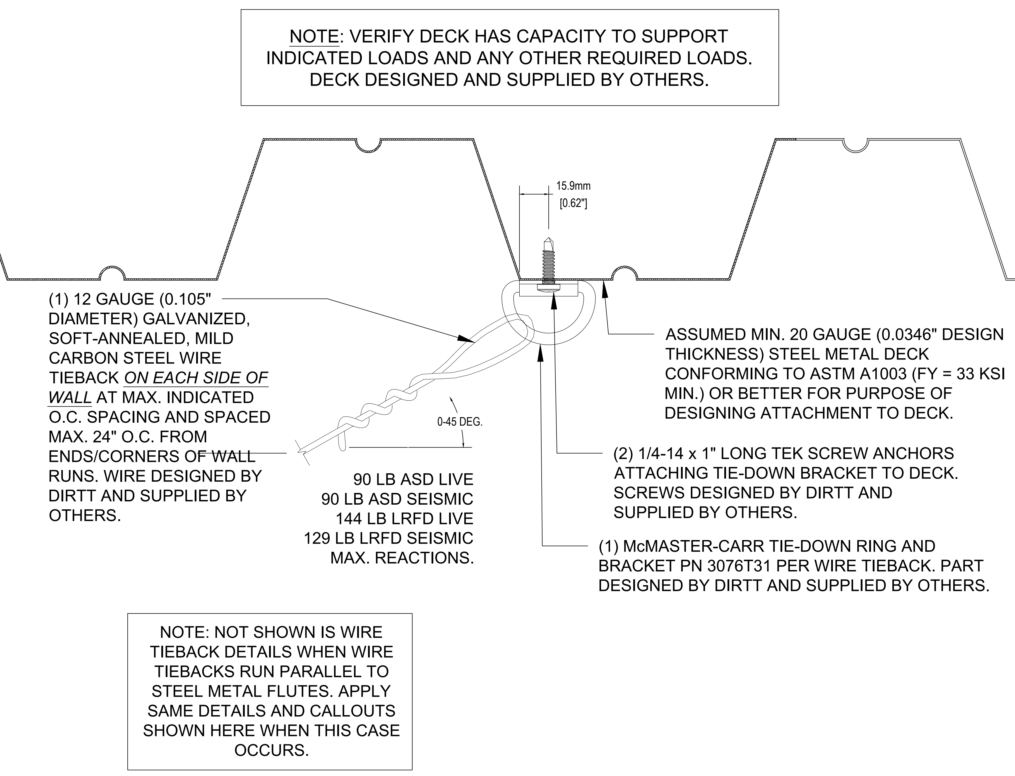
2 STEEL DECK - WIRE TIEBACKS DECK CONNECTION NTS
